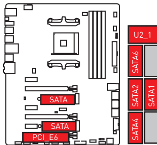
2xM.2 SATA SSDs + 4xSATA HDDs + 1xU.2 SSD + 1xPCI_E6 device
